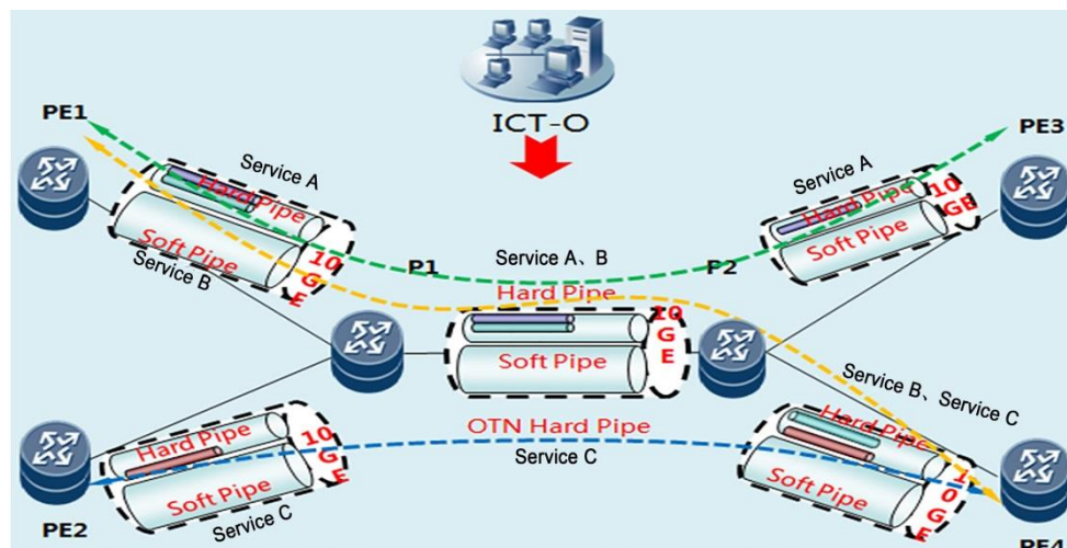
Figure 4-10 vNet private logic network
