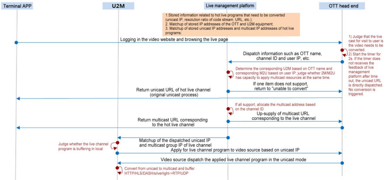
Figure 4-16 Treatment process of the U2M services
